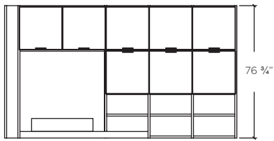
ELEVATION VIEW
