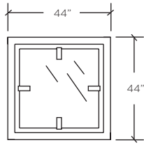
SQUARE COFFEE TABLE PLAN VIEW HEIGHT: 15"
